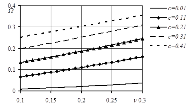
Figure 11 – Dependence of the maximum permissible relative length of the screw on the relative permissible power of the electric motor at different values of the critical slip of the electric motor
