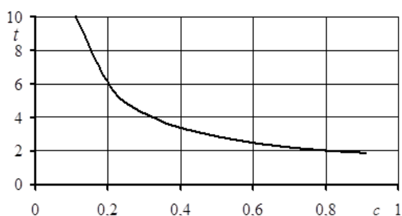
Figure 13 – Dependence of the maximum possible value of the relative permissible power of an electric motor on the actual critical slip of the electric motor
