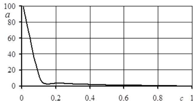
Figure 6 – Dependence of the inverse critical slip of an electric motor on the actual critical slip of an electric motor
