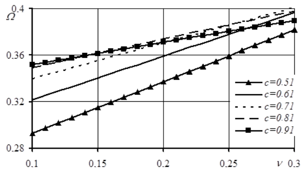
Figure 12 – Dependence of the value of the electromechanical coefficient on the relative permissible power of the electric motor at different values of the critical slip of the electric motor
