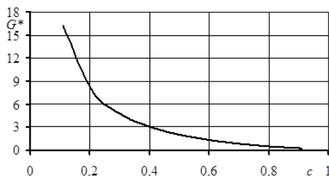
Figure 4 – Dependence of the maximum value of the relative volumetric flow rate of the transported material on the actual critical slip of the electric motor
