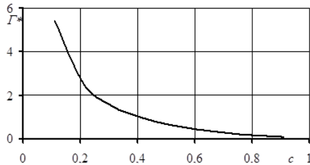
Figure 5 – Dependence of the maximum value of the relative power of the electric motor on the actual critical slip of the electric motor
