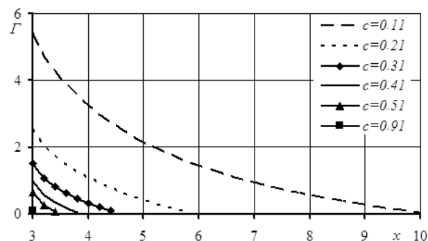
Figure 2 – Dependence of the relative power of the electric motor on the electromechanical parameter at different values of the critical slip of the electric motor
